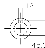
OUTPUT HOLLOW SHAFT
