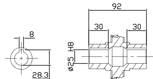
OUTPUT HOLLOW SHAFT
