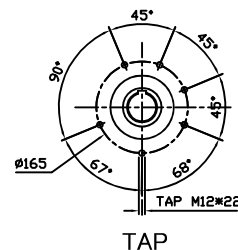
OUTPUT HOLLOW SHAFT
