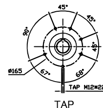
OUTPUT HOLLOW SHAFT
