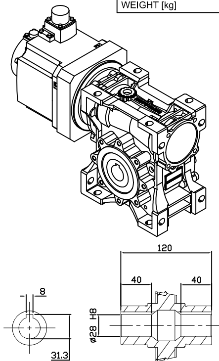
OUTPUT HOLLOW SHAFT
