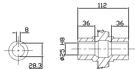
OUTPUT HOLLOW SHAFT
