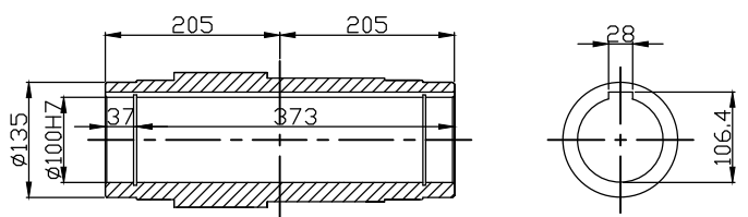
HOLLOW SHAFT
