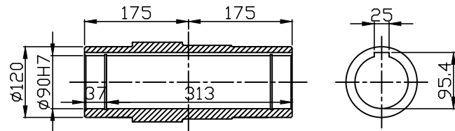
HOLLOW SHAFT
