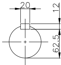
OUT-PUT SHAFT
