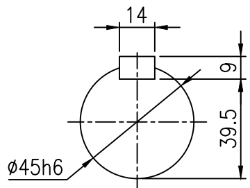
OUTPUT SHAFT
