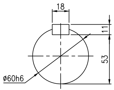
OUTPUT SHAFT
