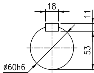
OUTPUT SHAFT
