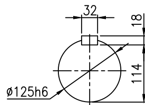
OUTPUT SHAFT
