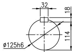
OUTPUT SHAFT
