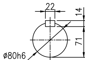
OUTPUT SHAFT
