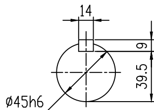
OUTPUT SHAFT
