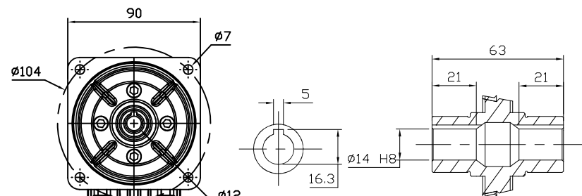
OUTPUT HOLLOW SHAFT
