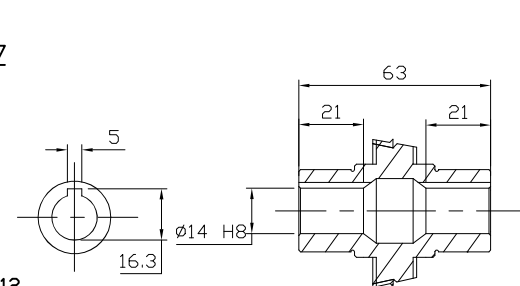
OUTPUT HOLLOW SHAFT
