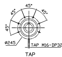
OUTPUT HOLLOW SHAFT
