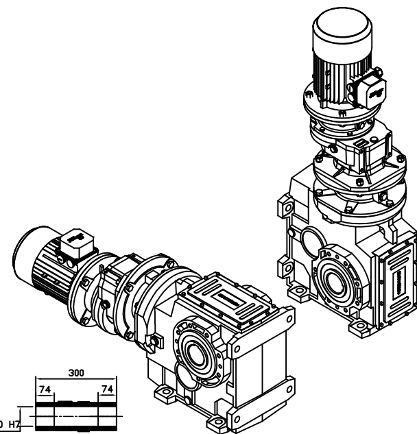
OUTPUT HOLLOW SHAFT
