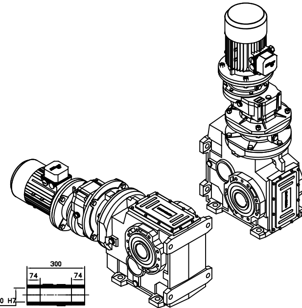
OUTPUT HOLLOW SHAFT
