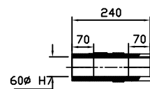
OUTPUT HOLLOW SHAFT
