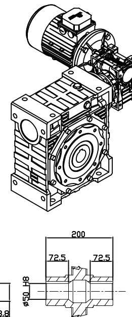
OUTPUT HOLLOW SHAFT
