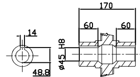
OUTPUT HOLLOW SHAFT
