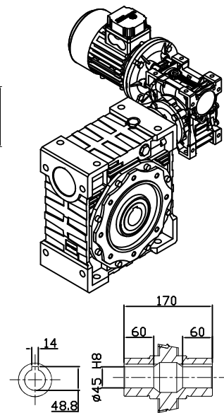
OUTPUT HOLLOW SHAFT
