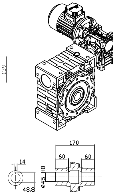
OUTPUT HOLLOW SHAFT
