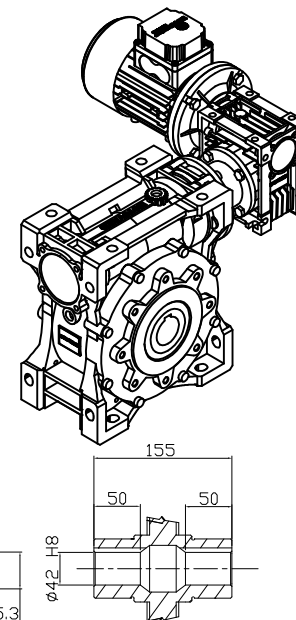
OUTPUT HOLLOW SHAFT
