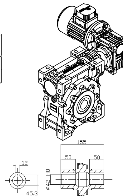
OUTPUT HOLLOW SHAFT
