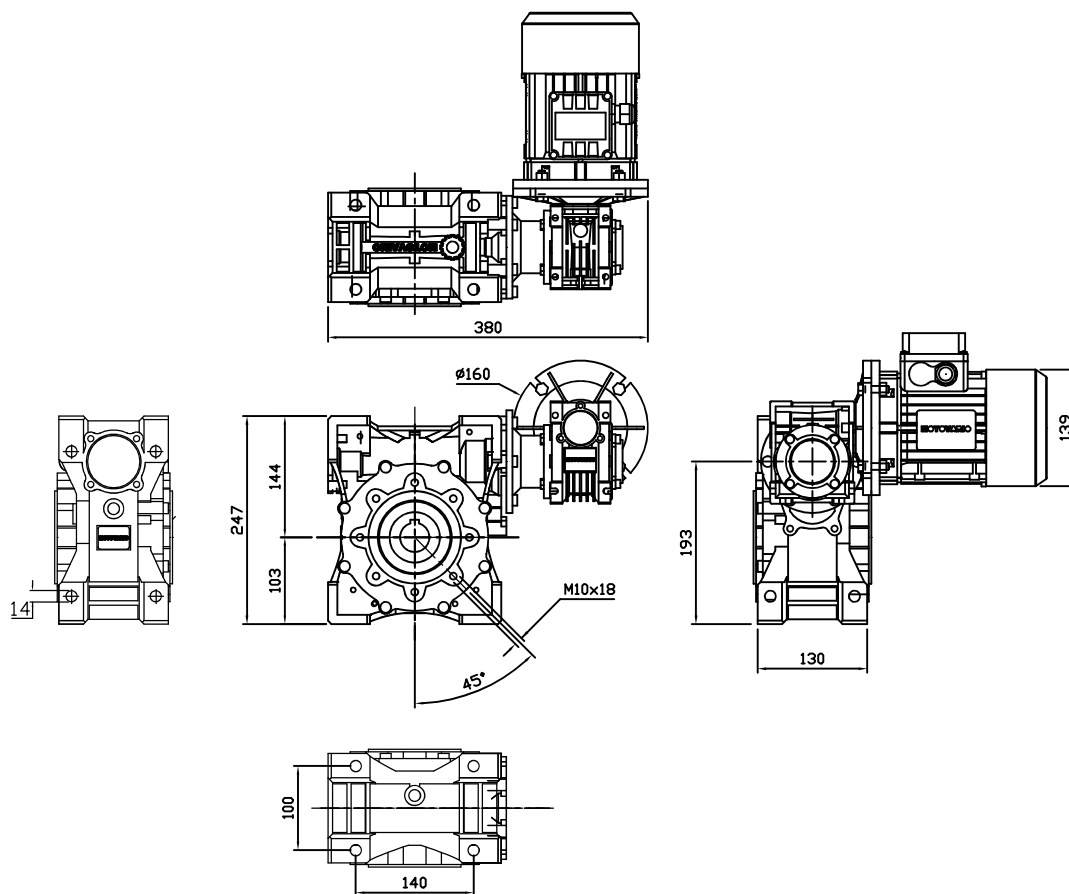
OUTPUT HOLLOW SHAFT
