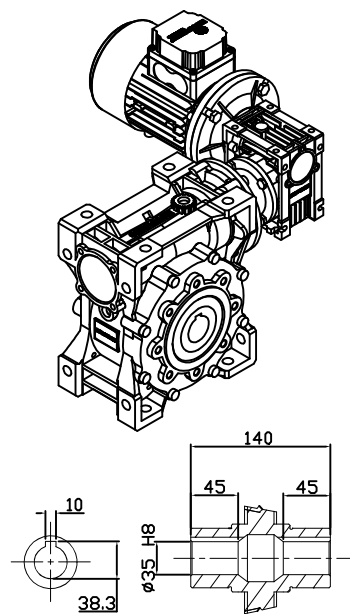
OUTPUT HOLLOW SHAFT
