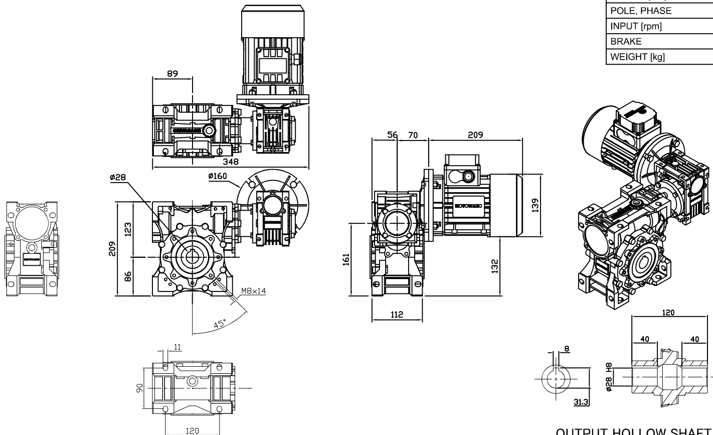
OUTPUT HOLLOW SHAFT
