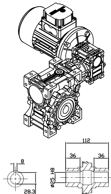
OUTPUT HOLLOW SHAFT
