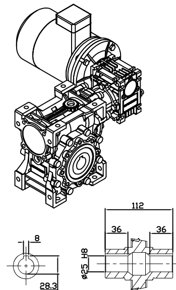
OUTPUT HOLLOW SHAFT
