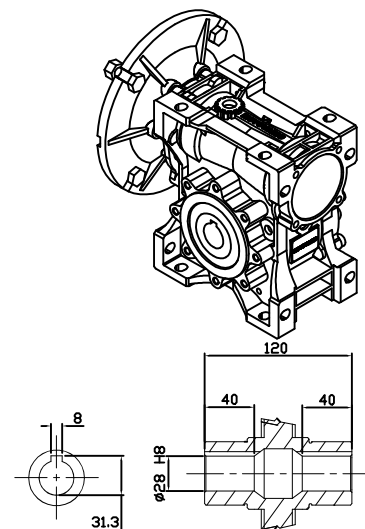
OUTPUT HOLLOW SHAFT
