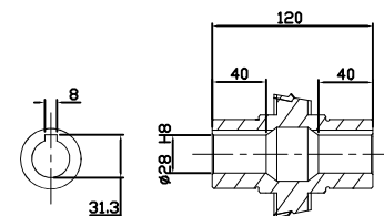
OUTPUT HOLLOW SHAFT
