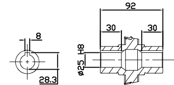
OUTPUT HOLLOW SHAFT
