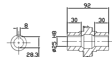
OUTPUT HOLLOW SHAFT
