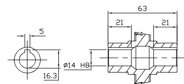
OUTPUT HOLLOW SHAFT
