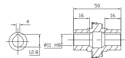
OUTPUT HOLLOW SHAFT
