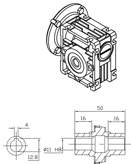
OUTPUT HOLLOW SHAFT
