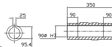
OUTPUT HOLLOW SHAFT
