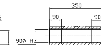
OUTPUT HOLLOW SHAFT
