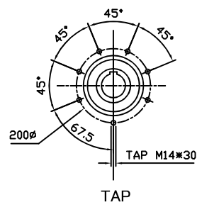
OUTPUT HOLLOW SHAFT
