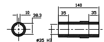
OUTPUT HOLLOW SHAFT
