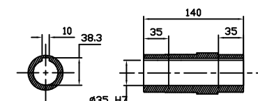
OUTPUT HOLLOW SHAFT
