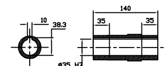
OUTPUT HOLLOW SHAFT
