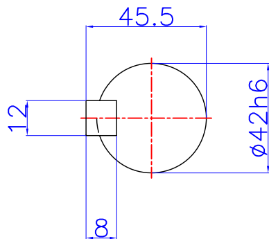
OUTPUT SHAFT
