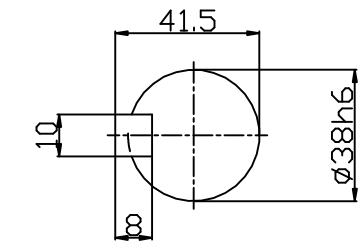
OUTPUT SHAFT
