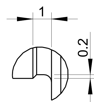
DETAIL A SCALE 10:1
