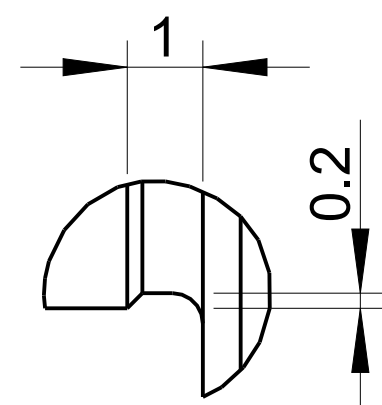
DETAIL A SCALE 10:1
